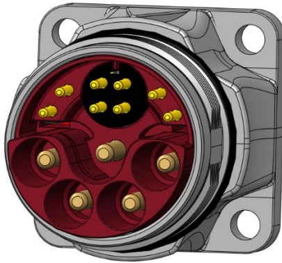
NEW revision pin insulation body
