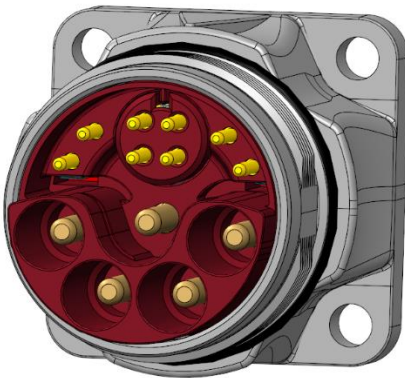
OLD revision pin insulation body
